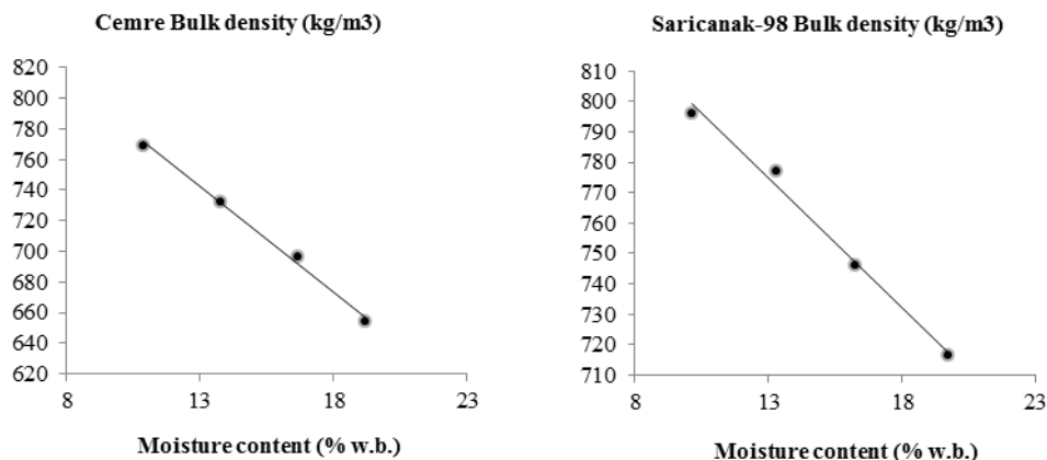
Figure 4. Effects of moisture content on bulk density
